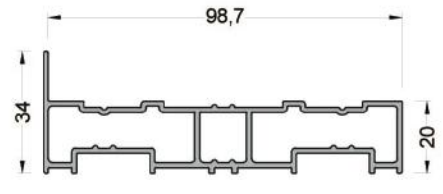
410-1103 ( 1,173 kg/mt ) GSAL100 KASA PROFİLİ
