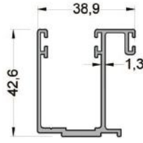
410-6007 (0,645 kg/mt ) GSAL100 SİSTEM RAY PROFİLİ
