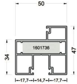
630-1104 (1,180 kg/mt) IP30F04 KASA PROFİLİ
