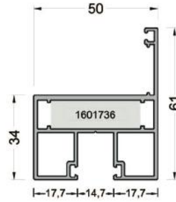
630-1103 (1,135 kg/mt) IP30F03 KASA PROFİLİ
