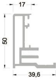
645-1101 (1,030 kg/mt ) IPA45F01 KASA PROFİLİ
