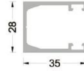
645-1201 (0,542 kg/mt ) IPA45F03 KASA PROFİLİ
