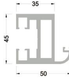
645-5101 (1,728 kg/mt ) IPA45F05 KASA PROFİLİ
