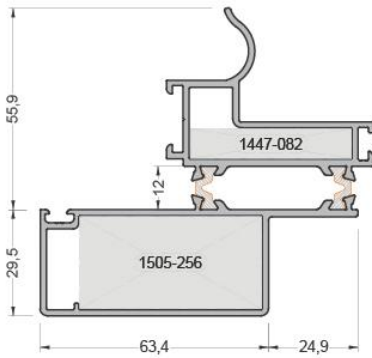
565-3101 ( 2,086 kg/mt ) SA65F01 KASA PROFİLİ
