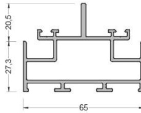
565-2102 ( 1,289 kg/mt ) SA65T02 YATAY PROFİL
