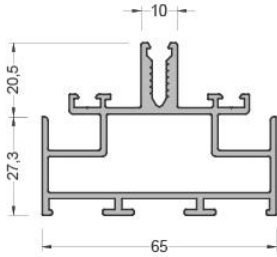
565-2101 ( 1,438 kg/mt ) SA65T01 YATAY PROFİL
