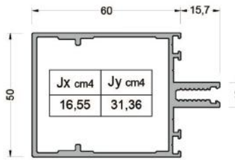
550-2205 ( 1,300 kg/mt ) W50T21 TRANSOM PROFİLİ
