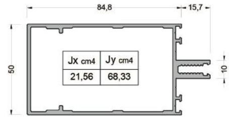
550-2201 ( 1,518 kg/mt ) W50T17 TRANSOM PROFİLİ
