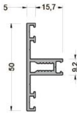
550-2101 ( 0,547 kg/mt ) W50T07 TRANSOM PROFİLİ
