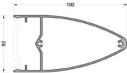
550-6202 ( 0,330 kg/mt ) W50P04 KAPAK PROFİLİ 16 mm
