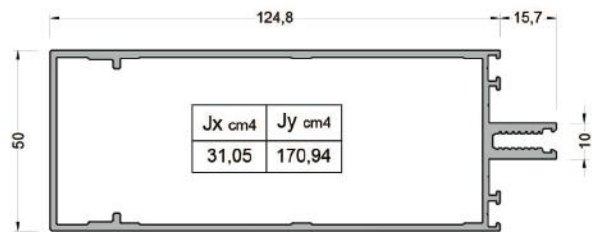
550-2203 ( 2,066 kg/mt ) W50T19 TRANSOM PROFİLİ
