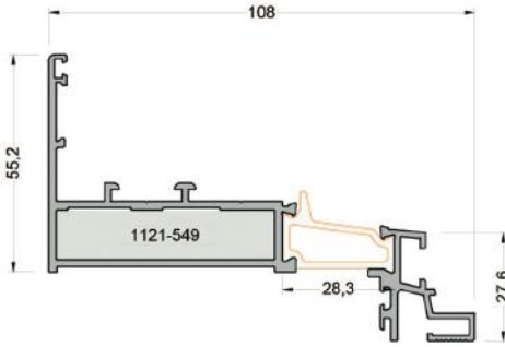
550-3102 ( 1,706 kg/mt ) W50F05 YALITIMLI KASA PROFİLİ
