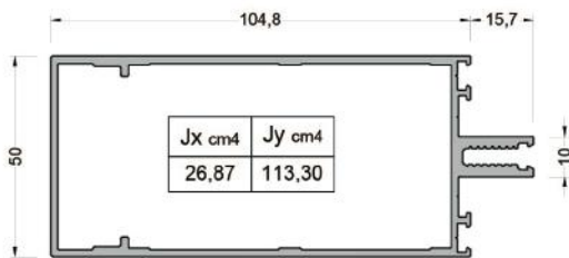
550-2202 ( 1,871 kg/mt ) W50T18 TRANSOM PROFİLİ
