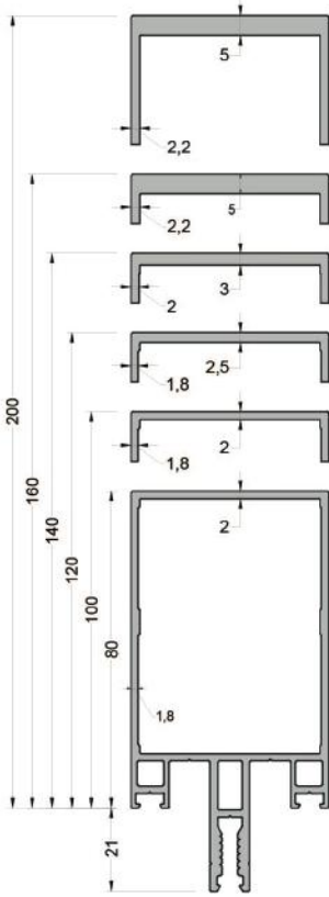
550-1206 ( 3,738 kg/mt ) W50M07 MÜLYON PROFİLİ
