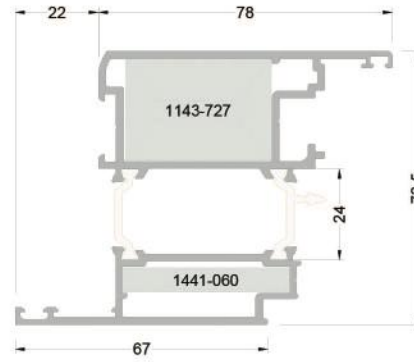
263-3610 ( 2,220 kg/mt ) T55V29 PVC KAPI KANAT PROFİLİ
