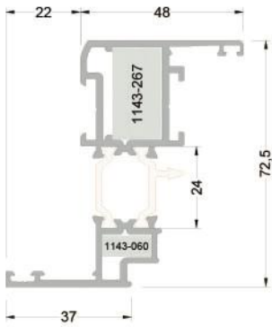
263-2401* ( 2,470 kg/mt ) T63M06 BAZA ORTAKAYIT PROFİLİ
