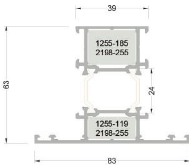
263-2203 ( 1,558 kg/mt ) T63M13 ORTA KAYIT PROFİLİ
