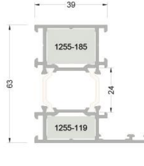
263-1202 ( 1,438 kg/mt ) T63F12 GENİŞ KASA PROFİLİ
