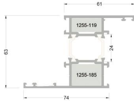
263-1501* ( 1,820 kg/mt ) T63F07 PERVAZLI KASA PROFİLİ
