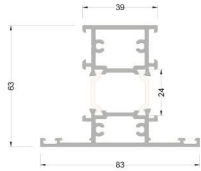
263-2202 ( 1,942 kg/mt ) T63M04 ORTA KAYIT PROFİLİ VİDALI
