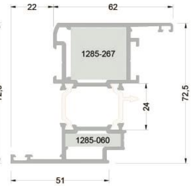
263-3201 ( 1,887 kg/mt ) T63V03 KANAT PROFİLİ
