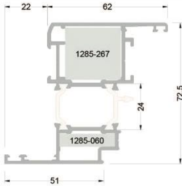
263-3203 ( 1,728 kg/mt ) T63V13 KANAT PROFİLİ
