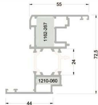
263-3609 ( 1,617 kg/mt ) T55V28 PVC KANAT PROFİLİ
