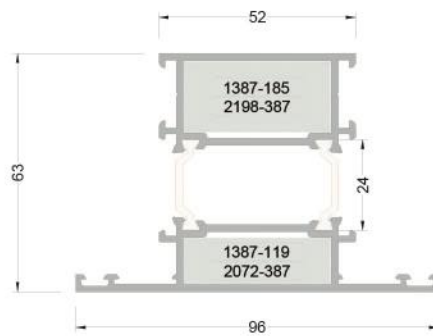
263-2301 ( 1,990 kg/mt ) T63M05 GENİŞ ORTA KAYIT PROFİLİ
