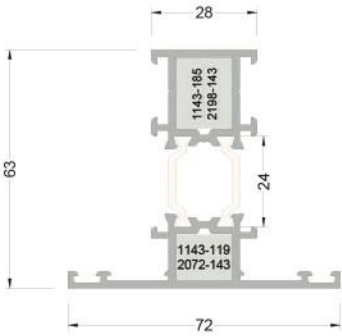
263-2101 ( 1,546 kg/mt ) T63M01 DAR ORTA KAYIT PROFİLİ
