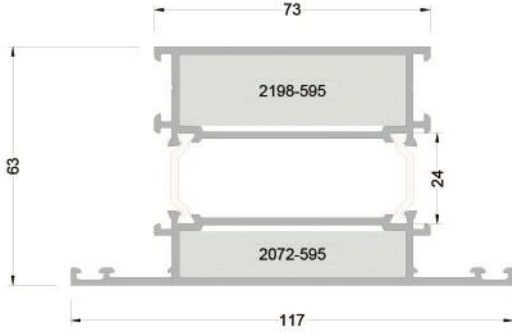
263-2401* ( 2,470 kg/mt ) T63M06 BAZA ORTAKAYIT PROFİLİ
