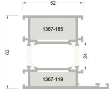
263-1301 ( 1,879 kg/mt ) T63F03 BAZA KASA PROFİLİ
