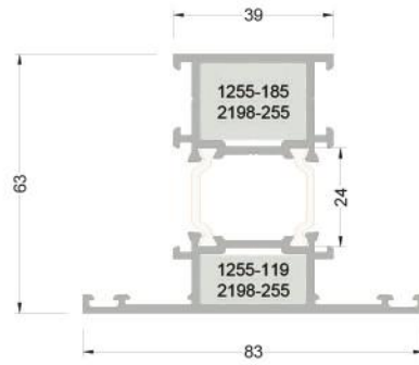
263-2201 ( 1,758 kg/mt ) T63M03 ORTA KAYIT PROFİLİ
