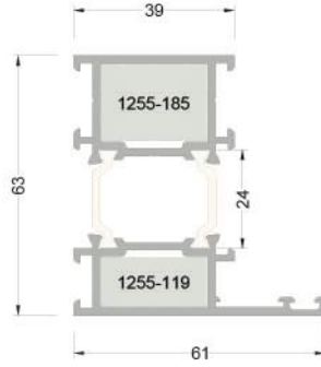
263-1201 ( 1,624 kg/mt ) T63F02 GENİŞ KASA PROFİLİ
