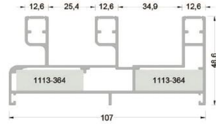
300-1203 ( 1,760 kg/mt ) SLA60F05 SİNEKLİK RAYLI KASA PROFİLİ
