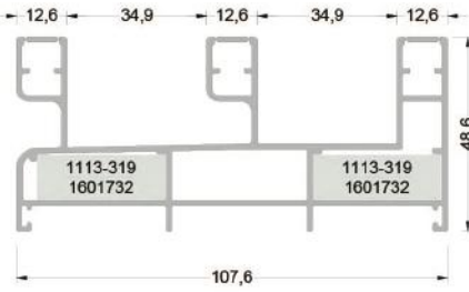
300-1301 ( 1,767 kg/mt ) SL60F03 3'LÜ KASA PROFİLİ
