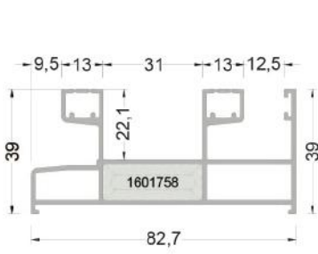
360-1202 ( 1,258 kg/mt ) 2 RAYLI KASA PROFİLİ
