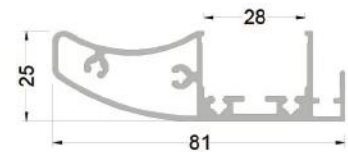
360-6003 ( 1,098 kg/mt ) TAKVİYELİ MİNİMAL KENET PROFİLİ
