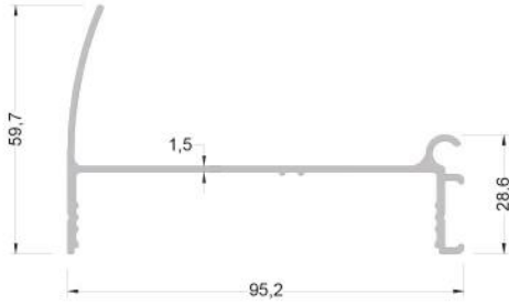
560-2101 ( 4,720 kg/mt ) DİKME PROFİLİ
