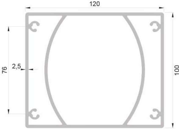
560-2101 ( 4,720 kg/mt ) DİKME PROFİLİ
