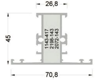
145-2101 ( 0,959 kg/mt ) WA45M01 DAR ORTA KAYIT PROFİLİ
