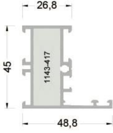
145-1101 ( 0,818 kg/mt ) WA45F01 DAR KASA PROFİLİ
