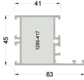
145-1201 ( 0,925 kg/mt ) WA45F02 KASA PROFİLİ
