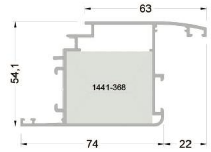
145-3401 ( 1,209 kg/mt ) WA45V02 KANAT PROFİLİ
