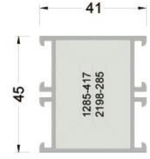
145-1202 ( 0,784 kg/mt ) WA45F04 KASA PROFİLİ
