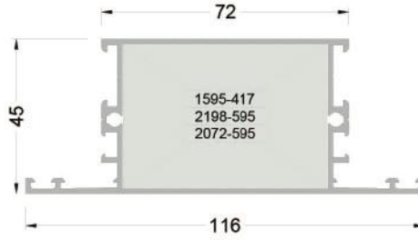
145-2301 ( 1,302 kg/mt ) WA45M03 BAZA ORTA KAYIT PROFİLİ
