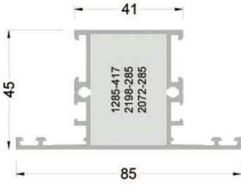
145-2201 ( 1,076 kg/mt ) WA45M02 ORTA KAYIT PROFİLİ
