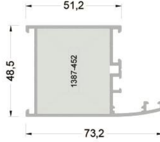
145-1302 ( 0,971 kg/mt ) WA45F06 GENİŞ KASA PROFİLİ
