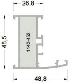
145-1102 ( 0,786 kg/mt ) WA45F05 DAR KASA PROFİLİ
