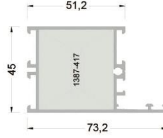
145-1301 ( 1,003 kg/mt ) WA45F03 GENİŞ KASA PROFİLİ
