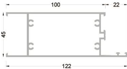
145-4401 ( 1,500 kg/mt ) WA45K01 ETEK PROFİLİ
