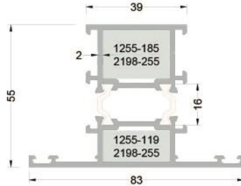
255-2201 (1,716 kg/mt.) T55M03 ORTA KAYIT PROFİLİ
