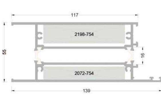
255-4401 ( 3,119 kg/mt ) T55K01 ETEK PROFİLİ
