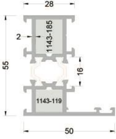
255-1101 (1,372 kg/mt.) T55F01 DAR KASA PROFİLİ
