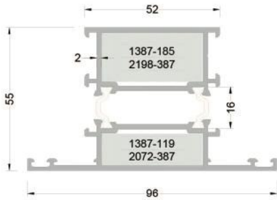
255-2301 (1,948 kg/mt.) T55M05 GENİŞ ORTA KAYIT PROFİLİ
