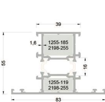
255-2203 (1,506 kg/mt.) T55M13 ORTA KAYIT PROFİLİ
