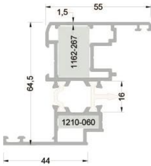
255-3609 ( 1,552 kg/mt ) T55V28 PVC KANAT PROFİLİ
