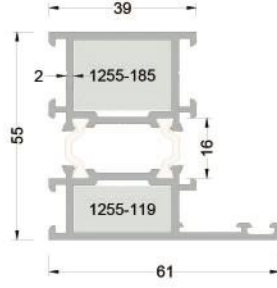
255-1201 (1,583 kg/mt.) T55F02 GENİŞ KASA PROFİLİ
