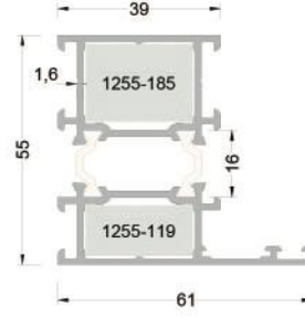
255-1202 (1,388 kg/mt.) T55F12 GENİŞ KASA PROFİLİ
