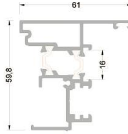
255-5101 ( 1,358 kg/mt ) T55A01 ÇİFT KANAT ADPTR PR.
