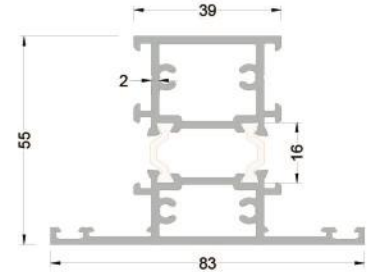
255-2202 (1,885 kg/mt.) T55M04 ORTA KAYIT PROFİLİ VİDALI
