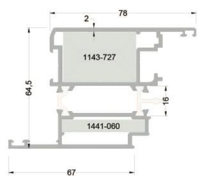
255-3610 ( 2,220 kg/mt ) T55V29 PVC KAPI KANAT PROFİLİ
