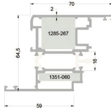
255-3601 ( 2,188 kg/mt ) T55V05 PVC KANAT PROFİLİ
