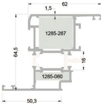
255-3203 ( 1,682 kg/mt ) T55V13 KANAT PROFİLİ
