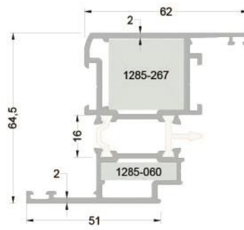
255-3201 ( 1,855 kg/mt ) T55V03 KANAT PROFİLİ
