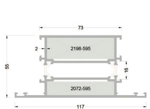
255-2401 (2,422 kg/mt.) T55M06 BAZA ORTA KAYIT PROFİLİ
