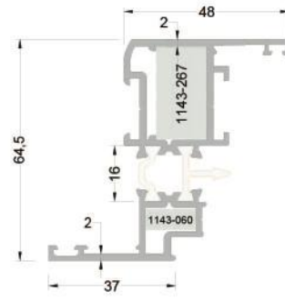
255-3102 ( 1,544 kg/mt ) T55V01 DAR KANAT PROFİLİ
