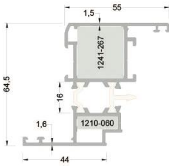
255-3205 ( 1,494 kg/mt ) T55V26 KANAT PROFİLİ
