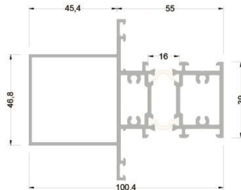
255-2502 (2,397 kg/mt.) T55M07 TAKVİYELİ ORTA KAYIT PROFİLİ
