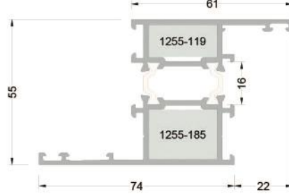
255-1501* (1,776 kg/mt.) T55F07 PERVAZLI KASA PROFİLİ
