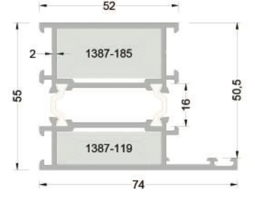
255-1301 (1,836 kg/mt.) T55F03 BAZA KASA PROFİLİ
