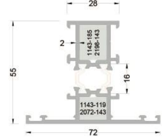
255-2101 (1,505 kg/mt.) T55M01 DAR ORTA KAYIT PROFİLİ
