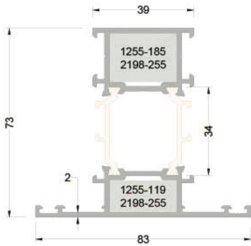
273-2201 (1,800 kg/mt) WAT73M03 ORTA KAYIT PROFİLİ
