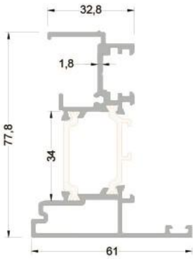
273-5101 ( 1,433 kg/mt ) WAT73A01 ÇİFT KANAT ADP. PR.
