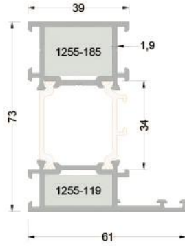
273-1201 (1,654 kg/mt) T55F02 KASA PROFİLİ 61MM
