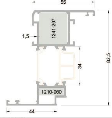
273-3205 (1,596 kg/mt) WAT73V26 KANAT PROFİLİ
