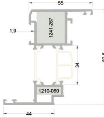
273-3204 (1,720 kg/mt) WAT73V25 KANAT PROFİLİ
