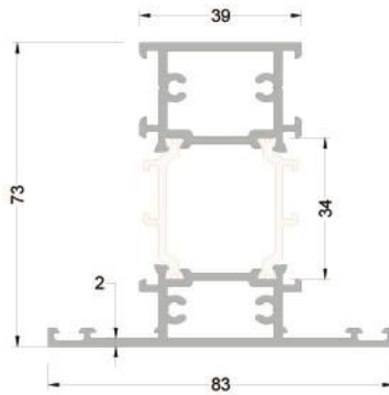
273-2202 (1,982 kg/mt) WAT73M04 ORTA KAYIT PROFİLİ VİDALI
