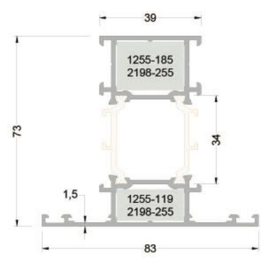
273-2203 (1,600 kg/mt) WAT73M13 ORTA KAYIT PROFİLİ
