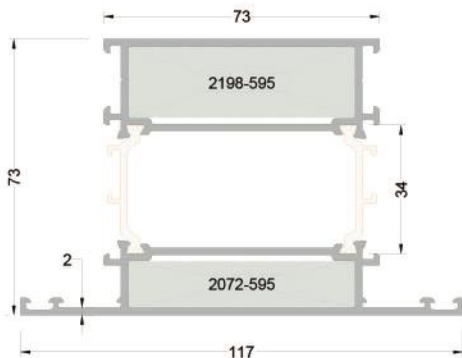
273-2401 (2,506 kg/mt) WAT73M06 ORTA KAYIT PROFİLİ
