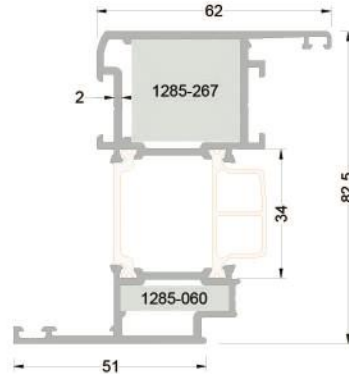
273-3203 (1,767 kg/mt) WAT73V13 KANAT PROFİLİ
