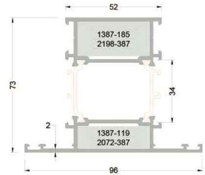
273-2301 (2,030 g/mt) WAT73M05 ORTA KAYIT PROFİLİ
