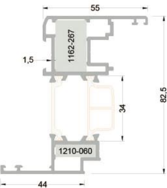
273-3609 (1,657 kg/mt) WAT73V28 PVC KANAT PROFİLİ
