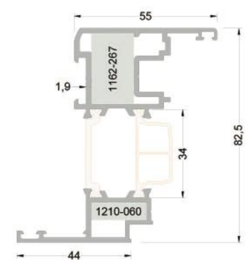
273-3608 (1,872 kg/mt) WAT73V27 PVC KANAT PROFİLİ
