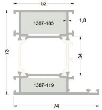
273-1301 (1,907 kg/mt) WAT73F03 BAZA KASA PROFİLİ
