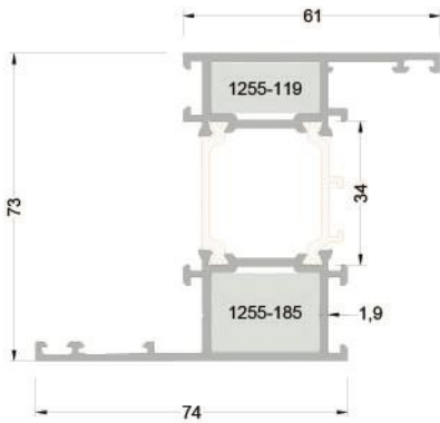
273-1501 (1,849 kg/mt) WAT73F07 PERVAZLI KASA PROFİLİ
