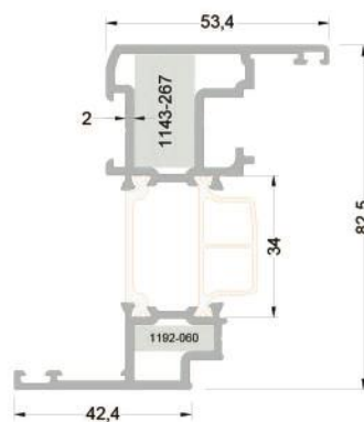
273-3604 (1,801 kg/mt) WAT73V17 KANAT PROFİLİ 53,4MM
