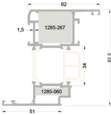
273-3201 (1,925 kg/mt) WAT73V03 KANAT PROFİLİ
