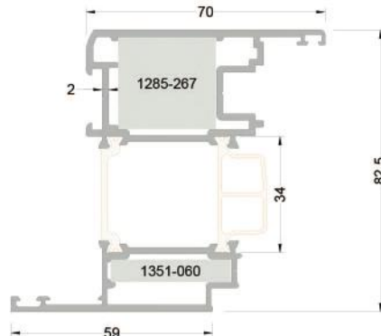
273-3601 (2,176 kg/mt) WAT73V05 PVC KANAT PROFİLİ
