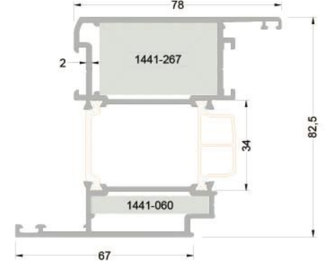
273-3401 (2,258 kg/mt) WAT73V09 KANAT PROFİLİ 78MM
