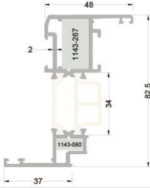
273-3102 (1,626 kg/mt) WAT73V01 DAR KANAT PROFİLİ
