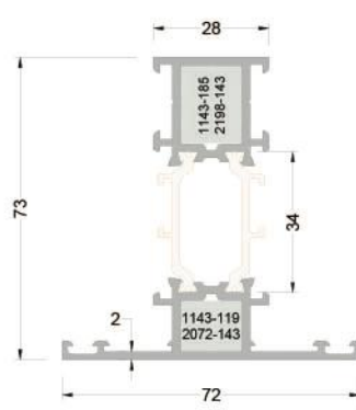
273-2101 (1,586 kg/mt) WAT73M01 ORTA KAYIT PROFİLİ
