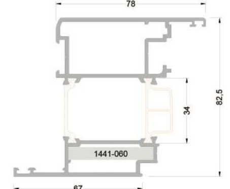
273-3610 (2,311 kg/mt) WAT73V29 PVC KAPI KANAT PROFİLİ
