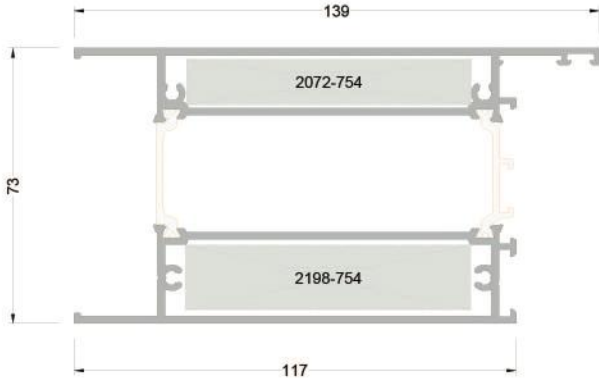
273-4401 ( 3,340 kg/mt ) WAT73K01 ETEK PROFİLİ
