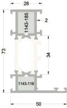
273-1101 (1,442 kg/mt) WAT73F01 KASA PROFİLİ
