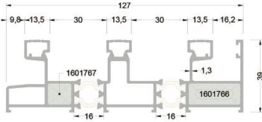
370-1201 ( 1,476 kg/mt ) 2 RAYLI KASA PROFİLİ
