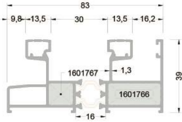
370-1201 ( 1,476 kg/mt ) 2 RAYLI KASA PROFİLİ
