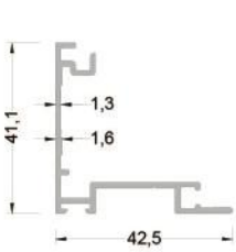
370-6002 ( 0,430 kg/mt ) KENET PROFİLİ
