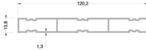
350-1202 (1,069 kg/mt ) SSA120 KASA PROFİLİ 120MM
