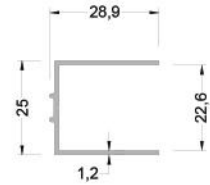
350-6001 (0,264 kg/mt ) SSA120 RAY PROFİLİ
