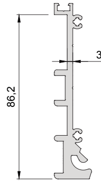
580-1204 ( 1,450 kg/mt ) SRA150M06 DUVAR BİTİM PROFİLİ
