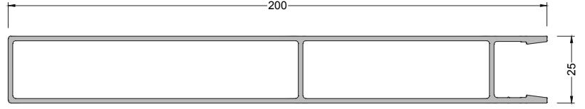
700-3106 ( 2,192 kg/mt ) ÇİT PANEL PROFİLİ
