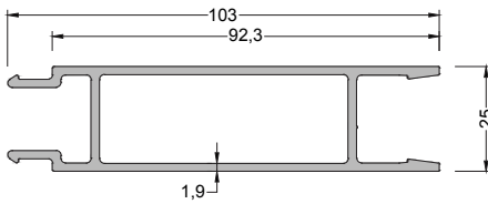
700-3103 ( 1,367 kg/mt ) ÇİT PANEL PROFİLİ
