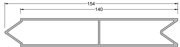
700-3104 ( 1,622 kg/mt ) ÇİT PANEL PROFİLİ
