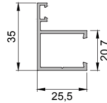
645-1202 ( 0,394 kg/mt ) IPA45F04 KASA PROFİLİ
