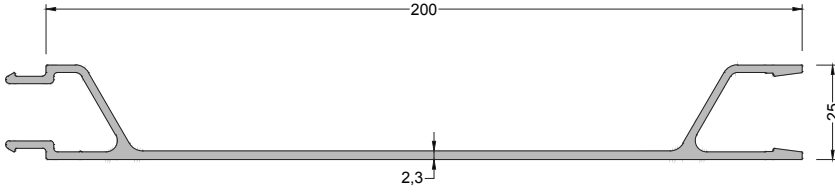
700-3110 ( 1,831 kg/mt ) ÇİT PANEL PROFİLİ
